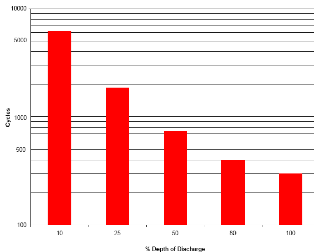
AGM Cycle Life vs. Depth of Discharge at +25°C (77°F) Based on BCI 2-hour Capacity
